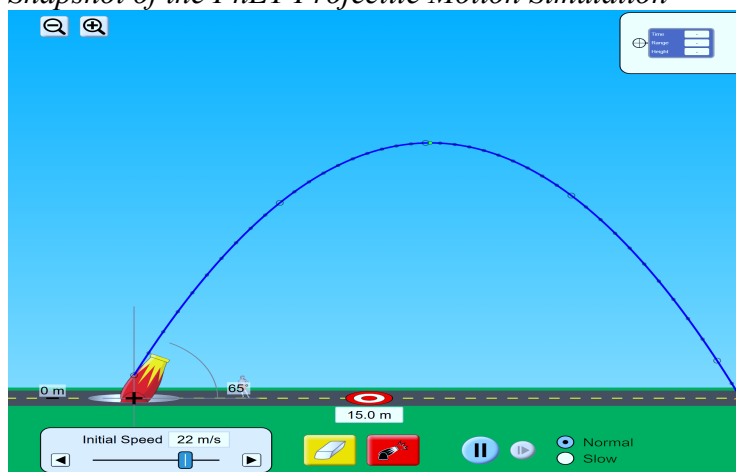
Figure 5 Snapshot of the PhET Projectile Motion Simulation
