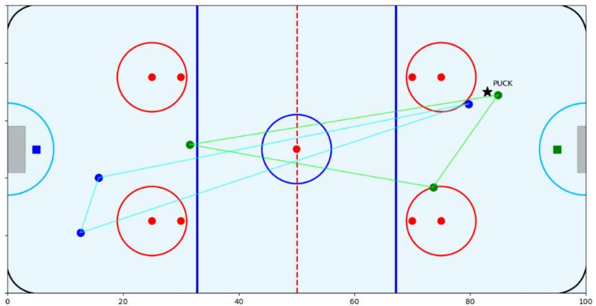
Figure 4 MARL Simulation
