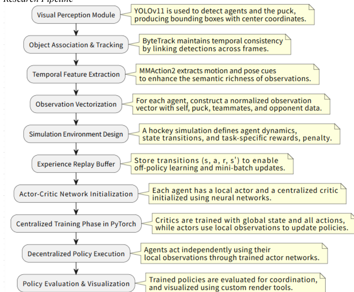
Figure 5 Research Pipeline
