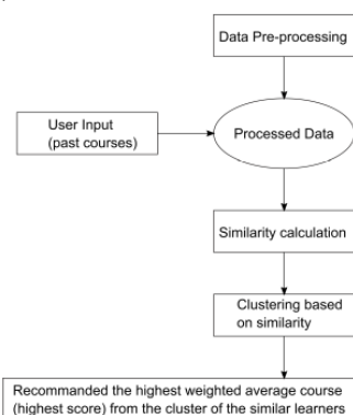
Fig. 1. Collaborative Filtering
