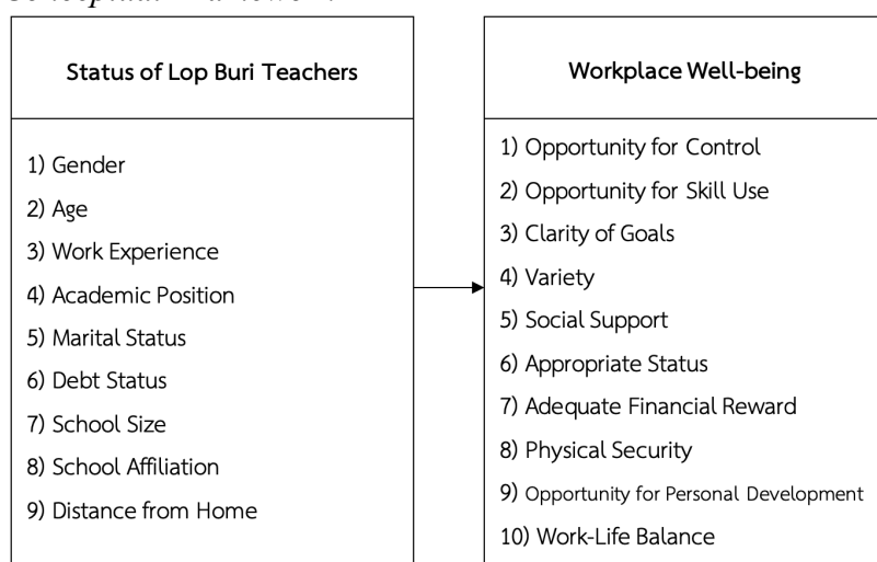
Figure 1 Conceptual Framework
