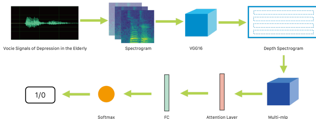
Figure 4. Speech recognition model of depression in the elderly people.
