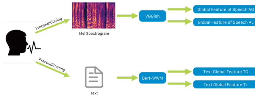
Figure 3. Speech global feature extraction.
